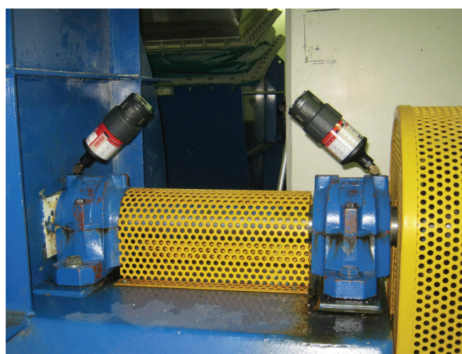
Application Fan support bearings Lubricator perma STAR VARIO 120 cm 3 Installation kit Direct mount
