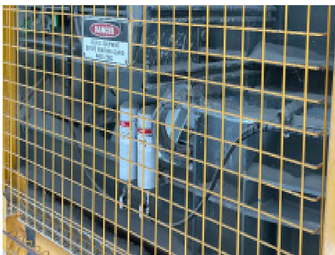
Application Travel wheels on conveyor tripper Lubricator perma STAR VARIO BLUETOOTH 250 cm³ Installation kit K230
