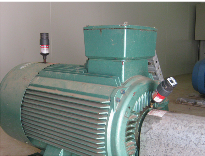
Application Electric motor Lubricator perma STAR VARIO 120 cm³ Installation kit Direct mount
